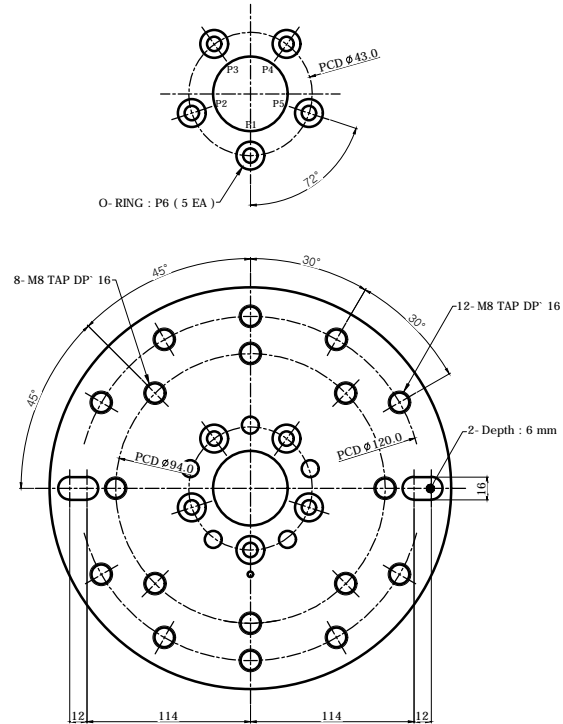
" C-Axis Spindle Dimensions ( 2 : 1 ) "
